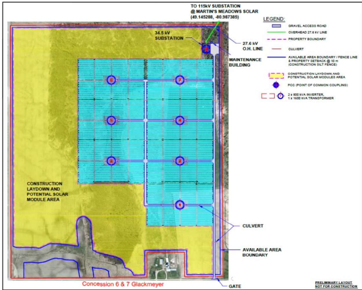
Figure 1: Site Layout
